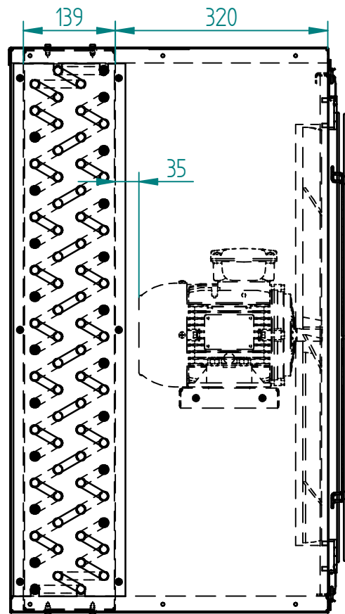
- Circuiting -
